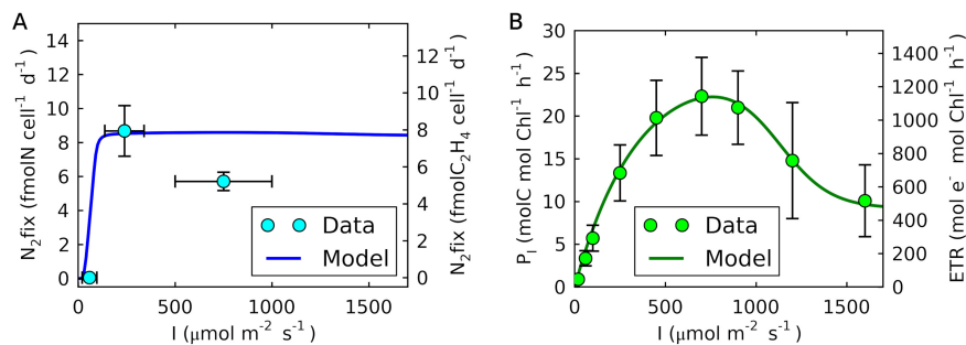
FIG 8 Experimental data and model simulation of the light dependence of daily integrated rates of \text{N}_2 fixation and photosynthesis of Crocosphaera . (A) Simulated light dependence of the \text{N}_2 fixation rate of Crocosphaera at 20% \text{O}_2 (left axis) compared with the acetylene reduction data obtained in this study (right axis). (B) Simulated light dependence of the photosynthesis rate (left axis) compared with the average daytime ETR (electron transfer rate) measured in this study (right axis) (measured in this study). Error bars represent the standard deviations of the samples. A temperature of 28°C was used.
