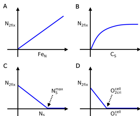
FIG 2 Schematics of how each factor influences N_{2fix} in the model. (A) Fe_N ; (B) C_S ; (C) N_S ; (D) O_2^{cell} . N_S^{max} is the maximum N storage capacity, and O_{2cri}^{cell} is the critical O 2 concentration.
